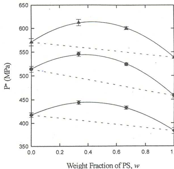
Figure 2. Characteristic pressures, P^* , in PS/TMPC mixtures as a function of PS weight fraction w . [ \diamond , \bullet , \blacktriangle ] correspond to values obtained by SL, FOV, and MCM, respectively. Solid lines represent the values obtained by fitting the points for each theory to eq 7, and the dotted lines represent additive values obtained using P^* of pure components. Error bars represent SE(P^*) shown in Table II.
